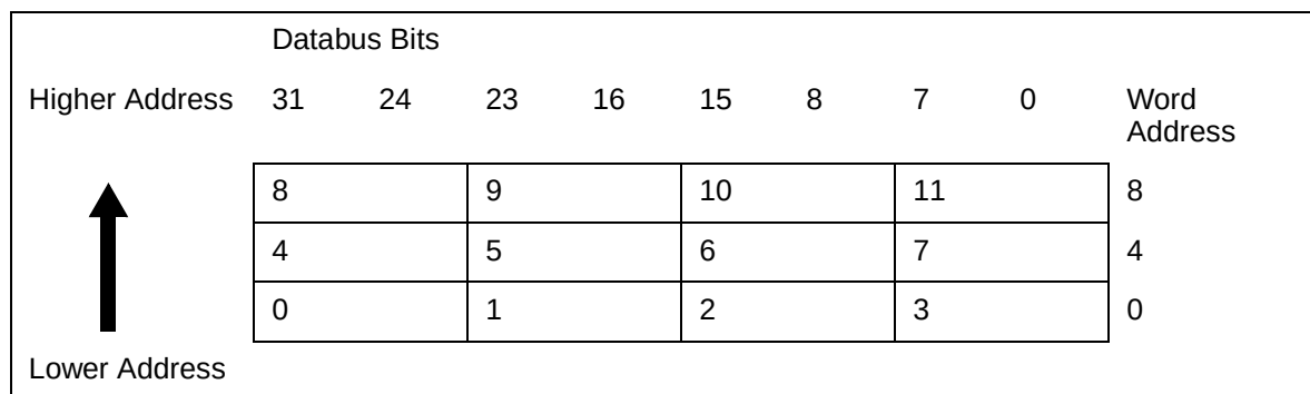
Figure 11-6: Big-endian addresses of bytes within words
